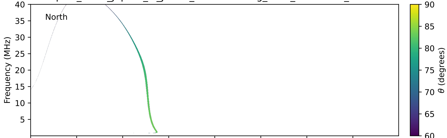
expres_earth_jupiter_io_jrm09_lossc-wid1deg_3kev_19980121_v11.cdf
