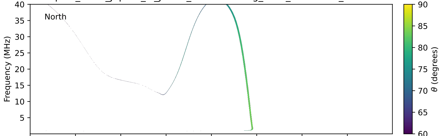
expres_earth_jupiter_io_jrm09_lossc-wid1deg_3kev_19980119_v11.cdf
