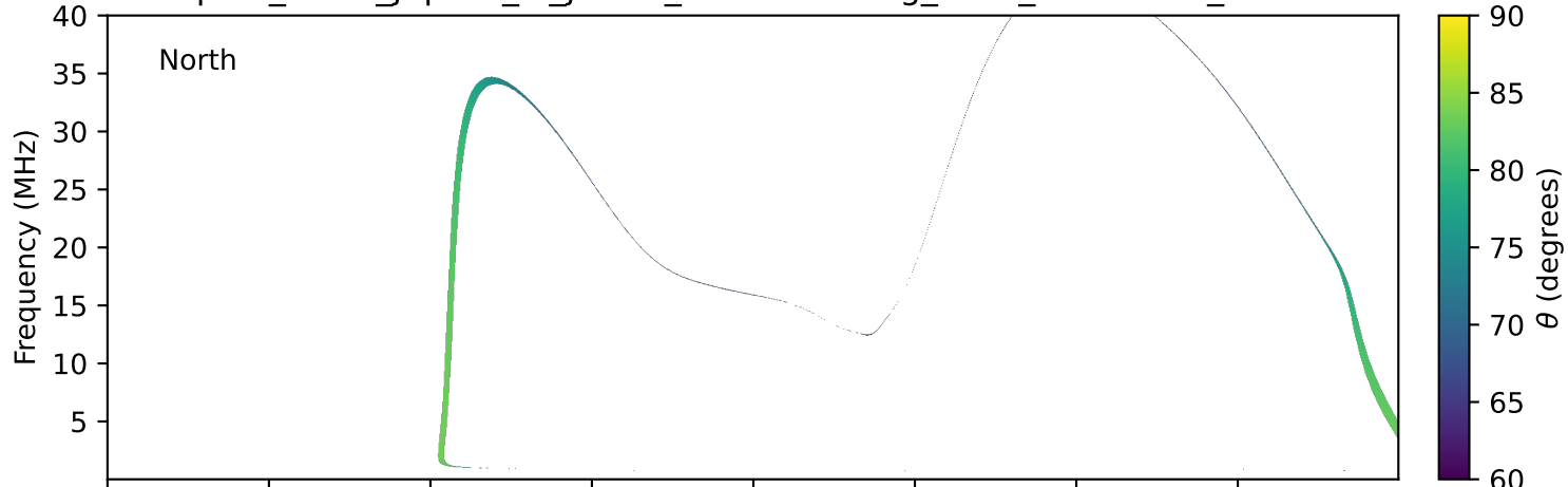
expres_earth_jupiter_io_jrm09_lossc-wid1deg_3kev_19980115_v11.cdf
