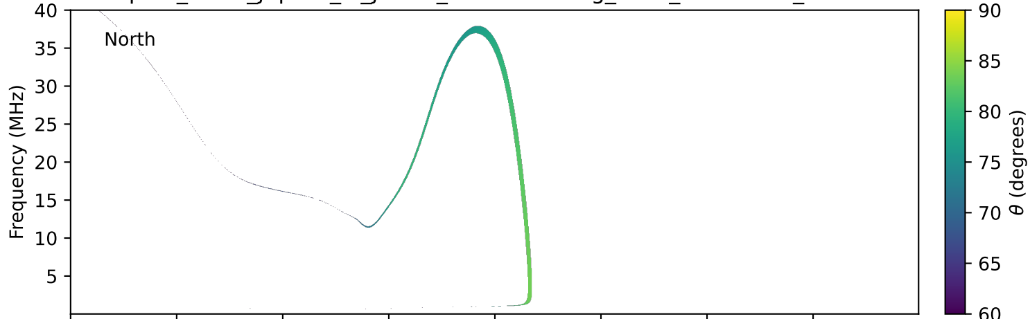
expres_earth_jupiter_io_jrm09_lossc-wid1deg_3kev_19980112_v11.cdf
