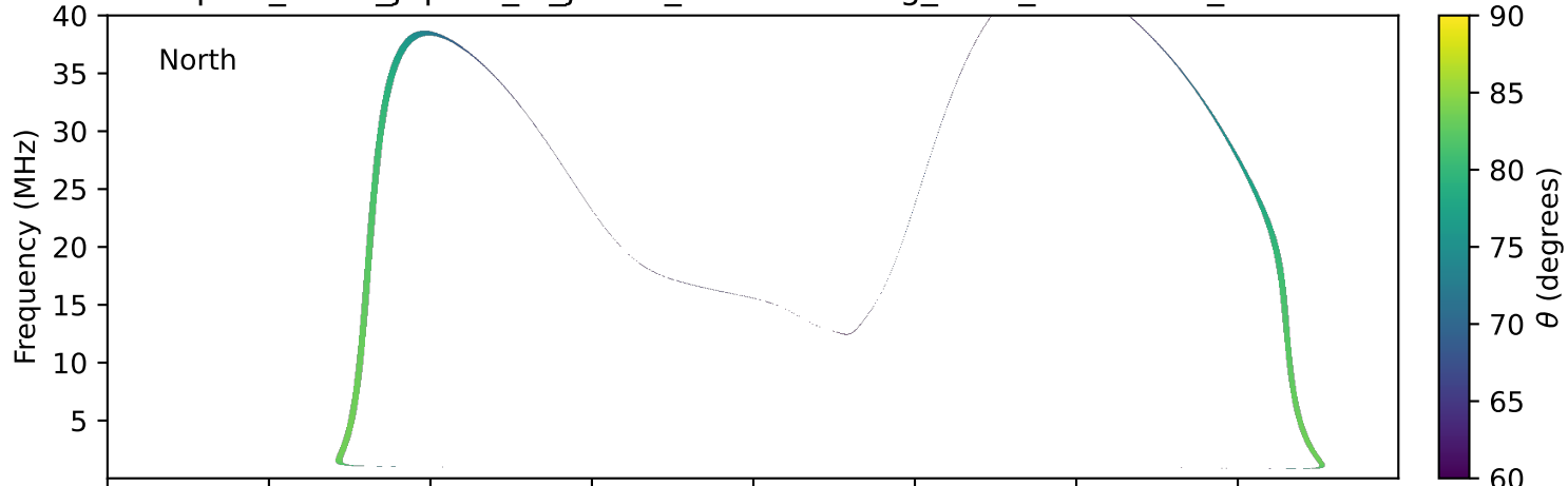
expres_earth_jupiter_io_jrm09_lossc-wid1deg_3kev_19980108_v11.cdf
