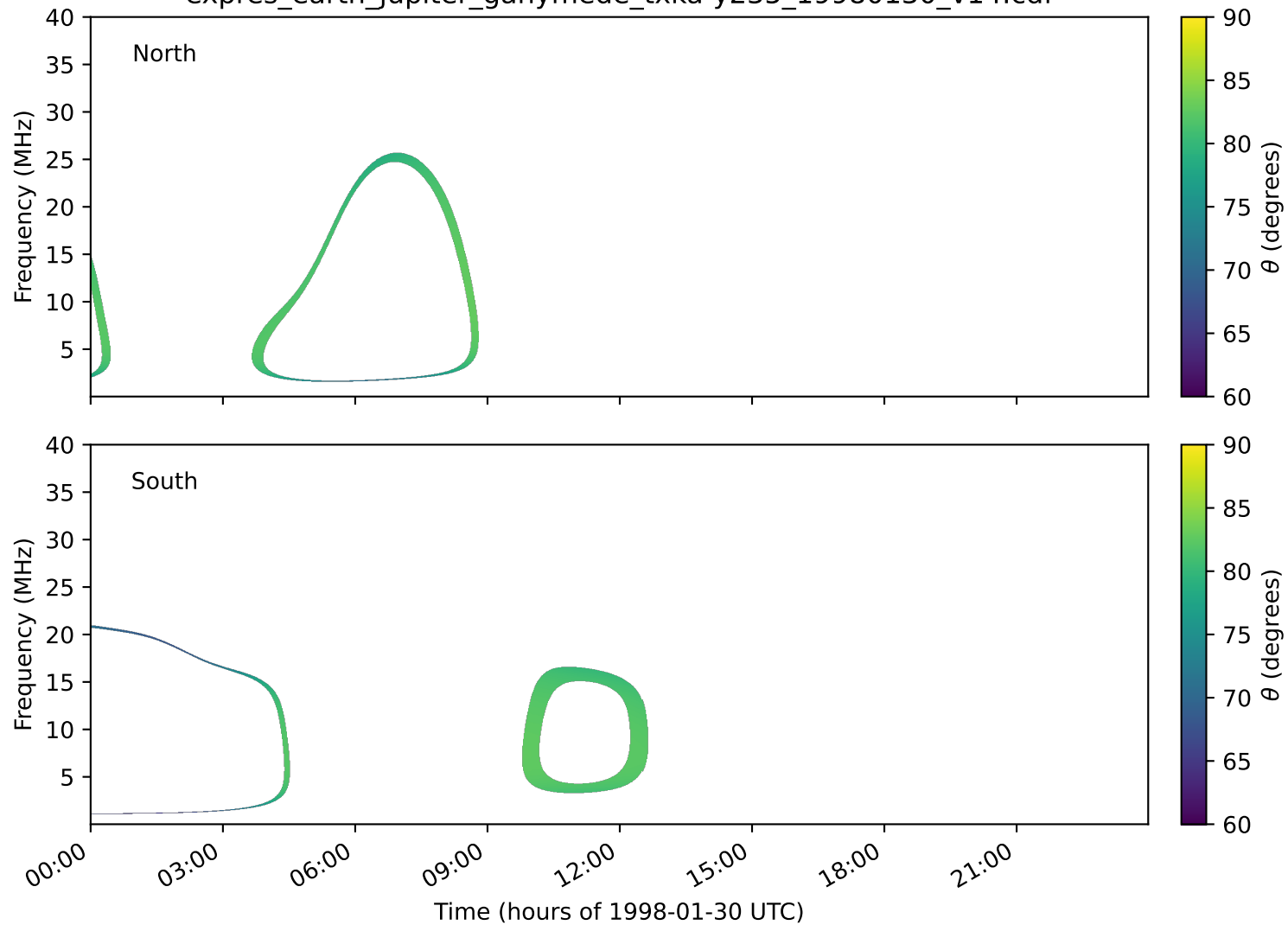
expres_earth_jupiter_ganymede_txka-y235_19980130_v14.cdf
