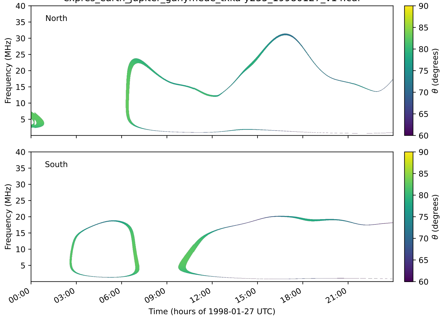
expres_earth_jupiter_ganymede_txka-y235_19980127_v14.cdf
