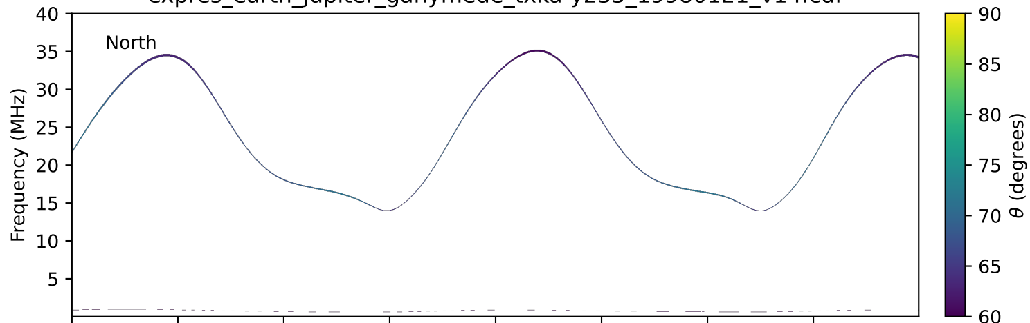
expres_earth_jupiter_ganymede_txka-y235_19980121_v14.cdf
