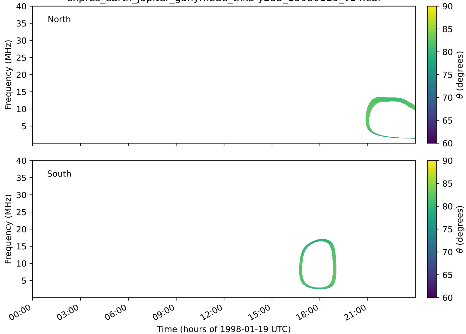
expres_earth_jupiter_ganymede_txka-y235_19980119_v14.cdf
