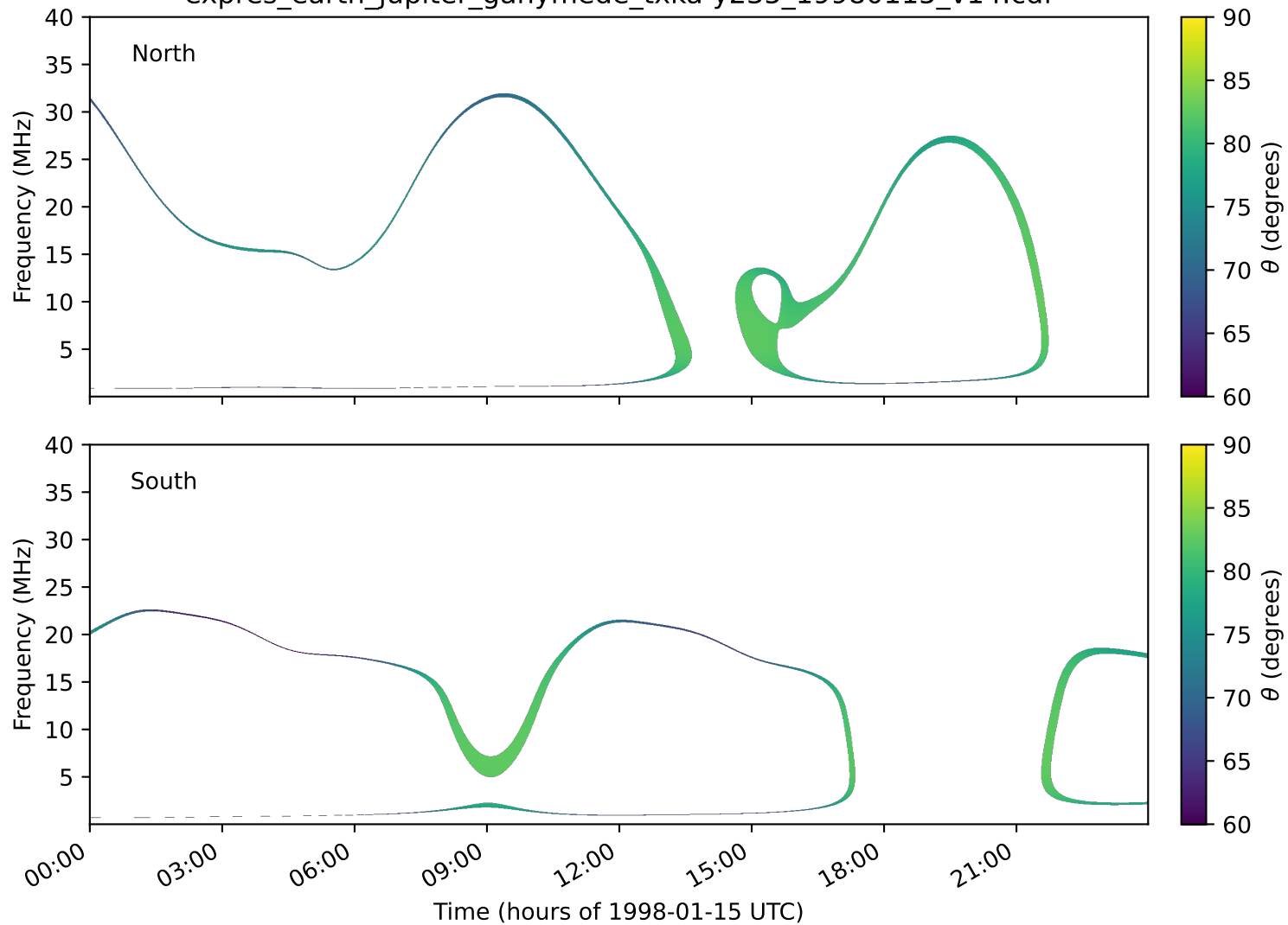
expres_earth_jupiter_ganymede_txka-y235_19980115_v14.cdf
