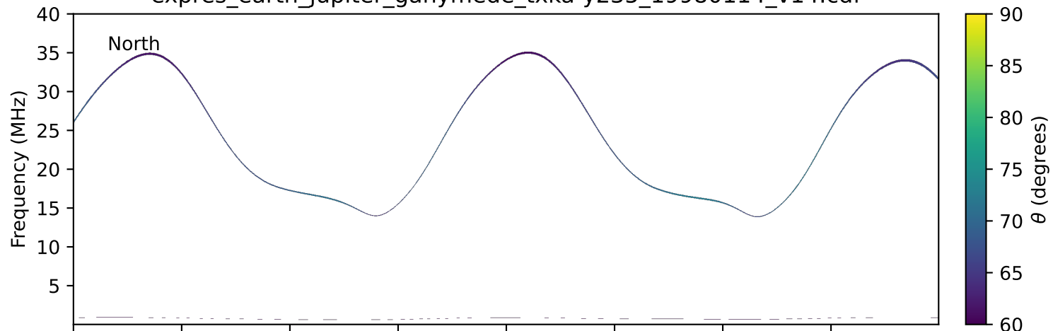
expres_earth_jupiter_ganymede_txka-y235_19980114_v14.cdf
