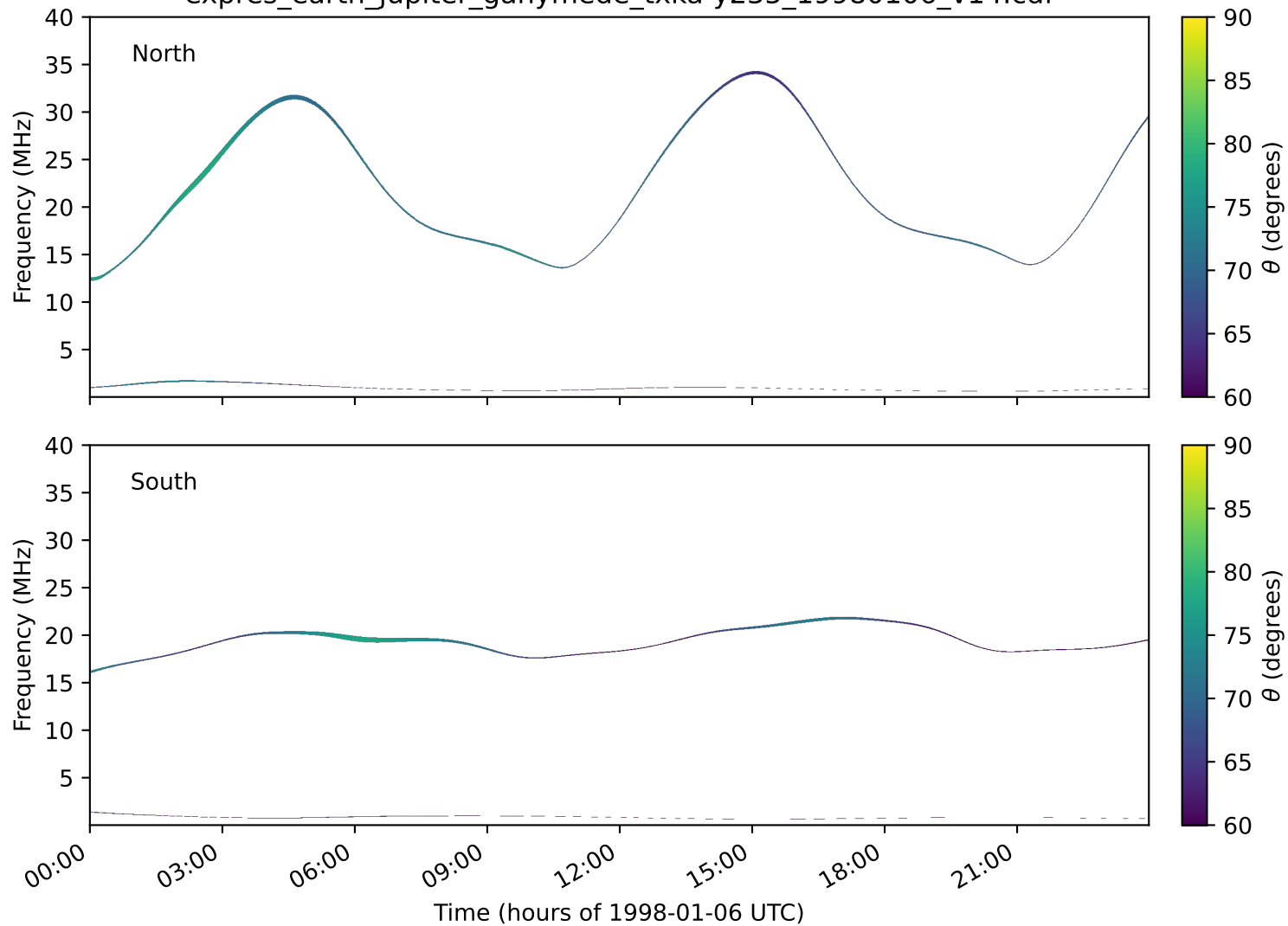
expres_earth_jupiter_ganymede_txka-y235_19980106_v14.cdf
