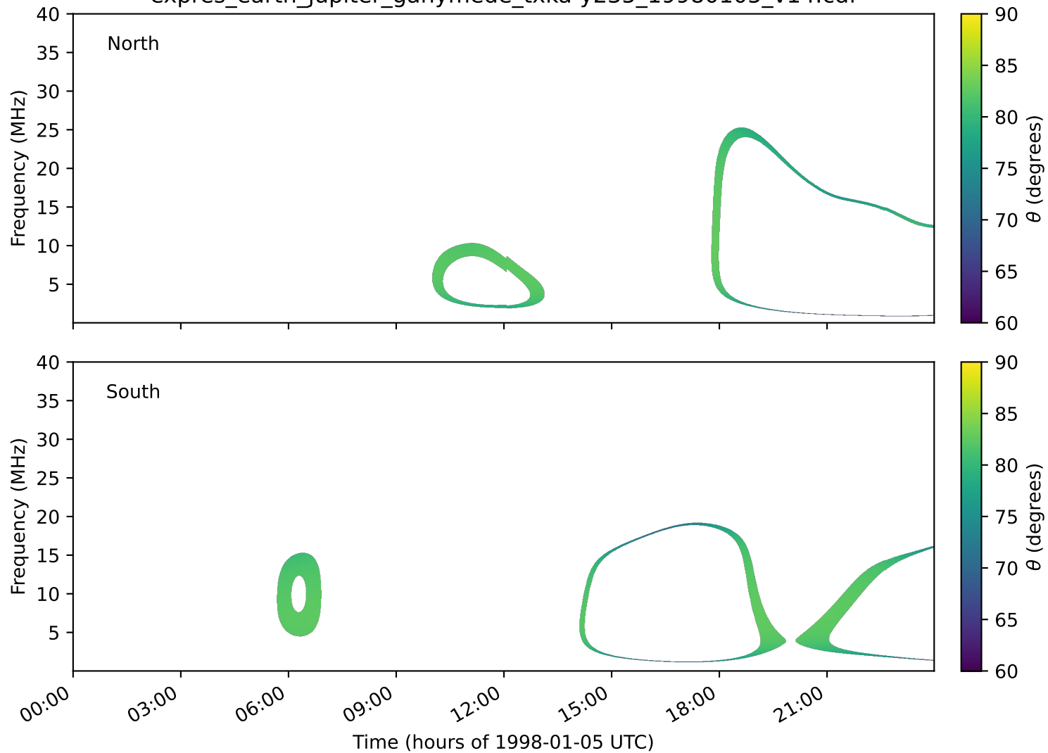
expres_earth_jupiter_ganymede_txka-y235_19980105_v14.cdf
