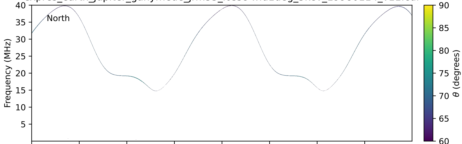
expres_earth_jupiter_ganymede_jrm33_lossc-wid1deg_3kev_19980114_v11.cdf
