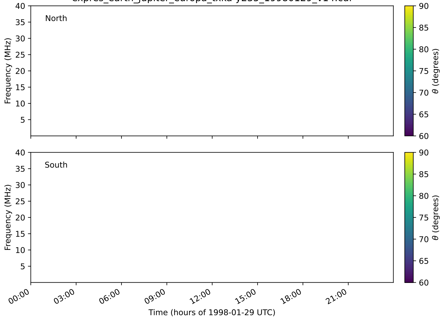
expres_earth_jupiter_europa_txka-y235_19980129_v14.cdf
