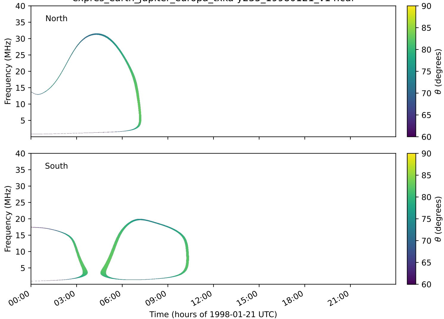
expres_earth_jupiter_europa_txka-y235_19980121_v14.cdf
