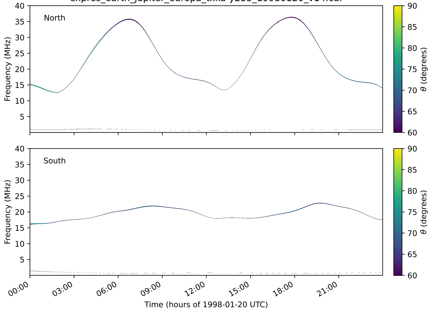
expres_earth_jupiter_europa_txka-y235_19980120_v14.cdf
