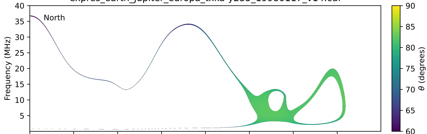
expres_earth_jupiter_europa_txka-y235_19980117_v14.cdf
