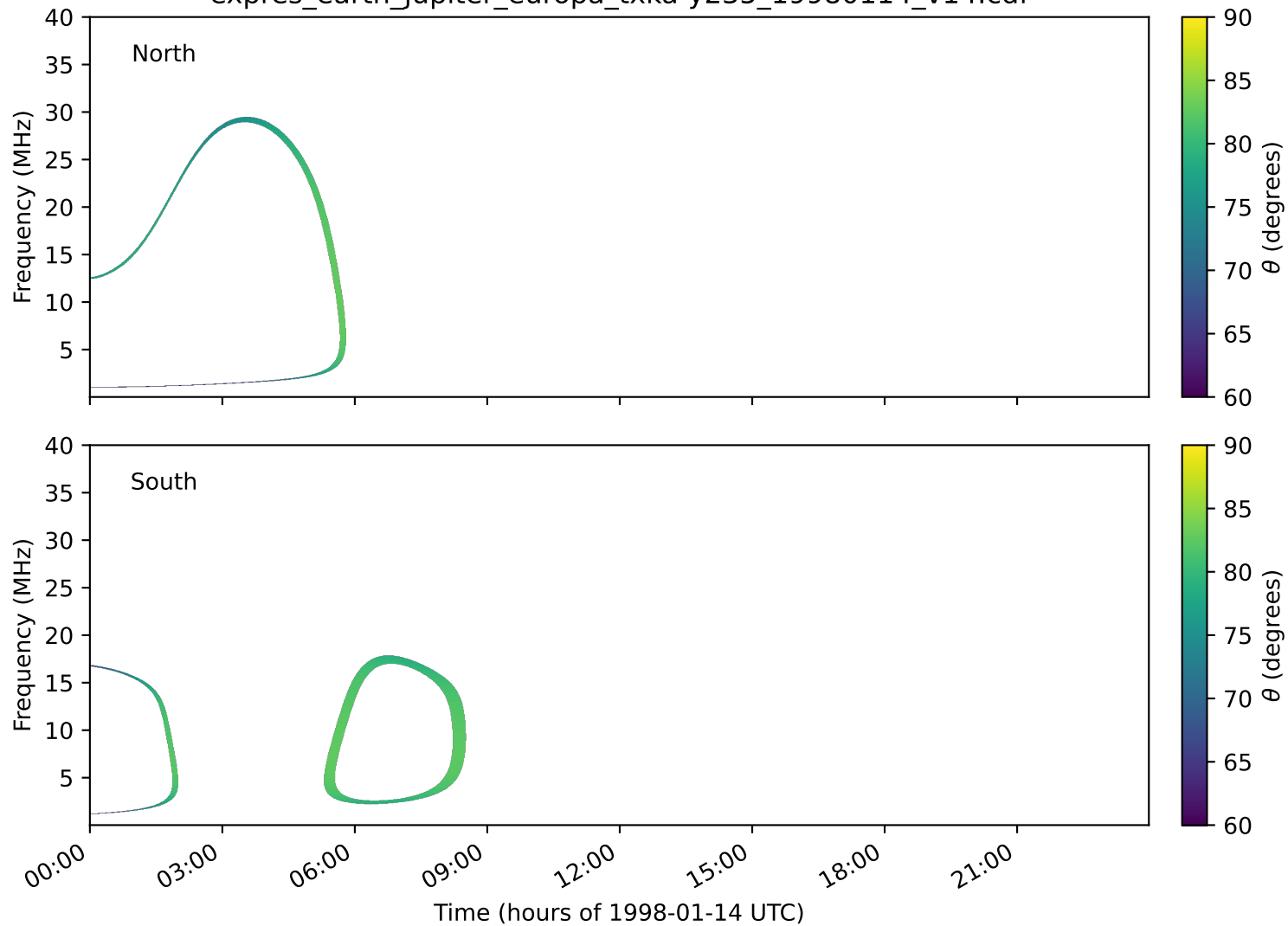
expres_earth_jupiter_europa_txka-y235_19980114_v14.cdf
