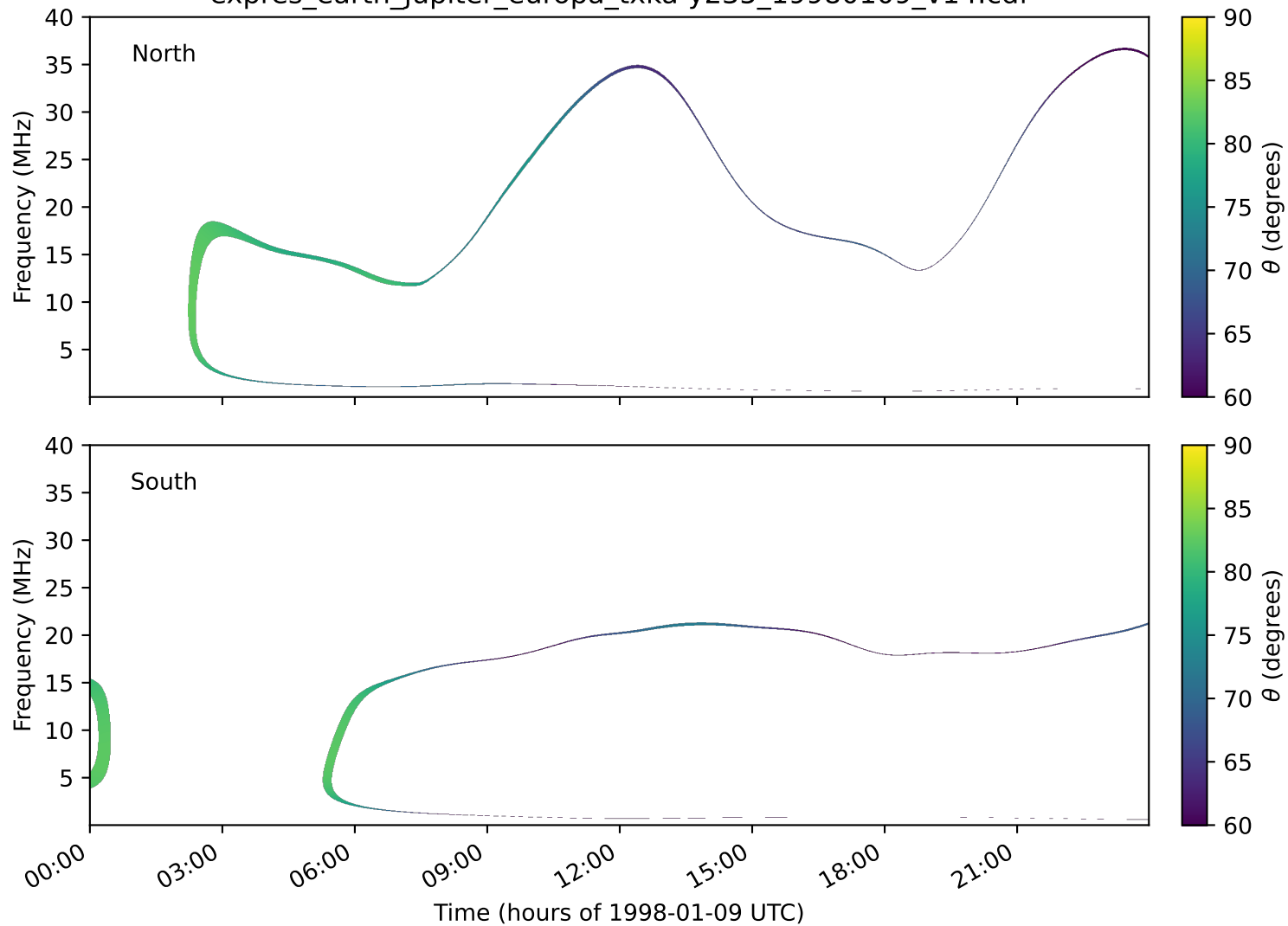
expres_earth_jupiter_europa_txka-y235_19980109_v14.cdf
