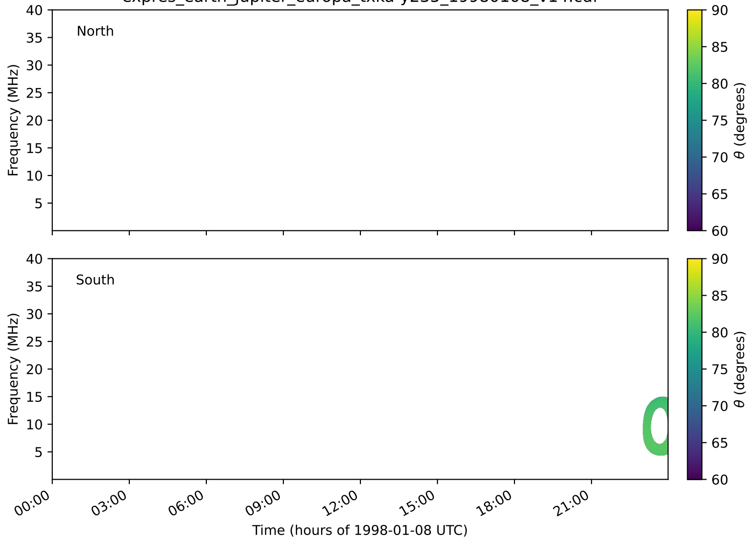
expres_earth_jupiter_europa_txka-y235_19980108_v14.cdf
