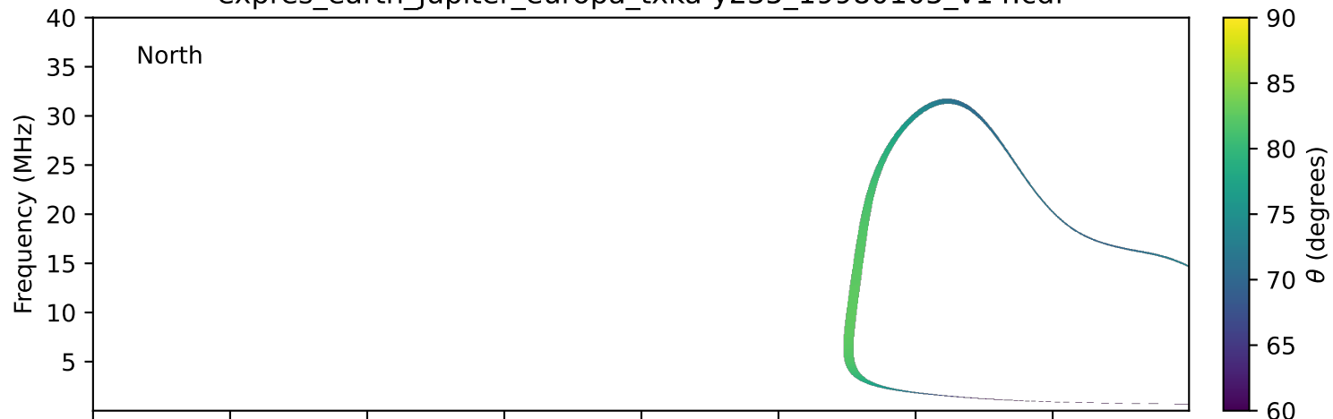
expres_earth_jupiter_europa_txka-y235_19980105_v14.cdf
