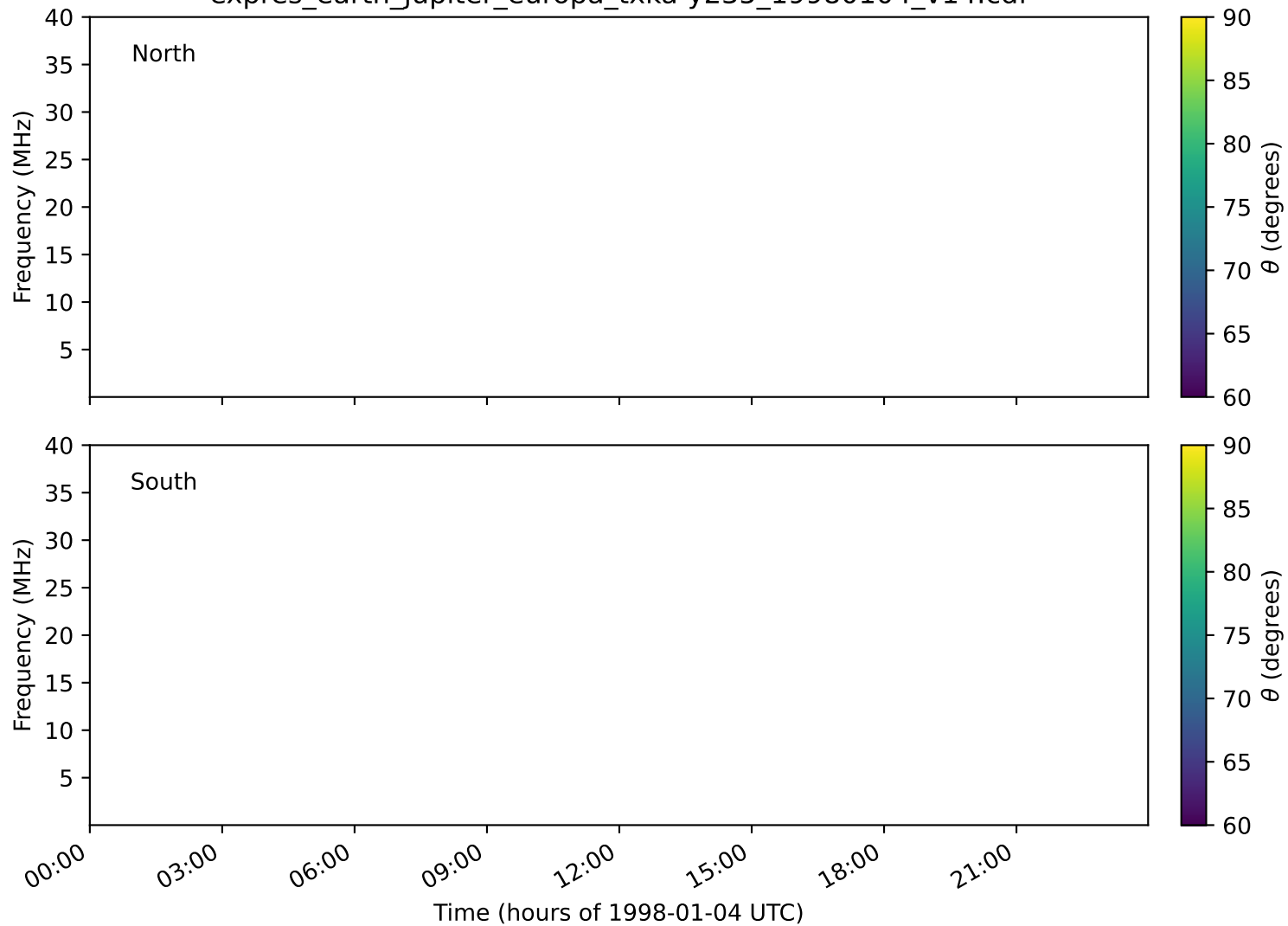
expres_earth_jupiter_europa_txka-y235_19980104_v14.cdf
