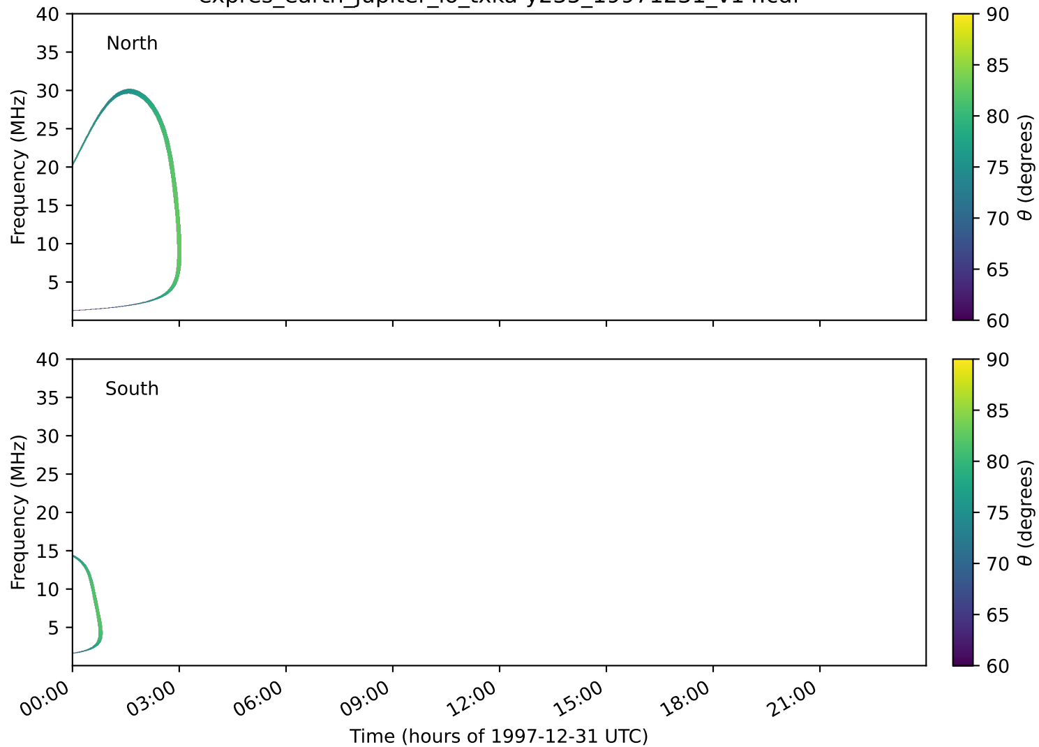
expres_earth_jupiter_io_txka-y235_19971231_v14.cdf
