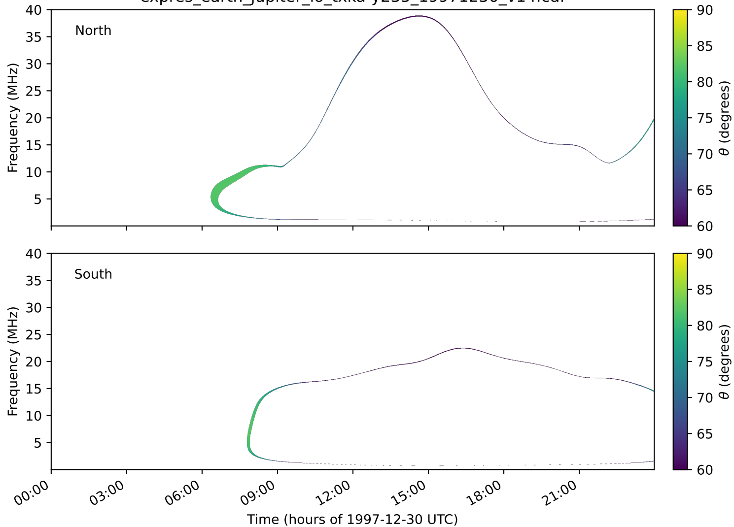
expres_earth_jupiter_io_txka-y235_19971230_v14.cdf
