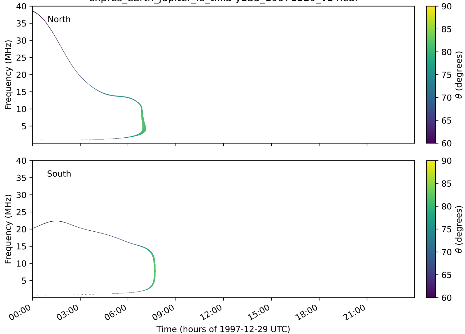
expres_earth_jupiter_io_txka-y235_19971229_v14.cdf
