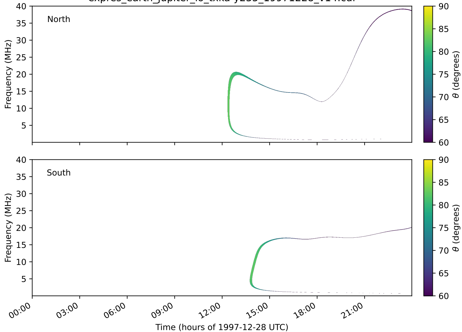
expres_earth_jupiter_io_txka-y235_19971228_v14.cdf
