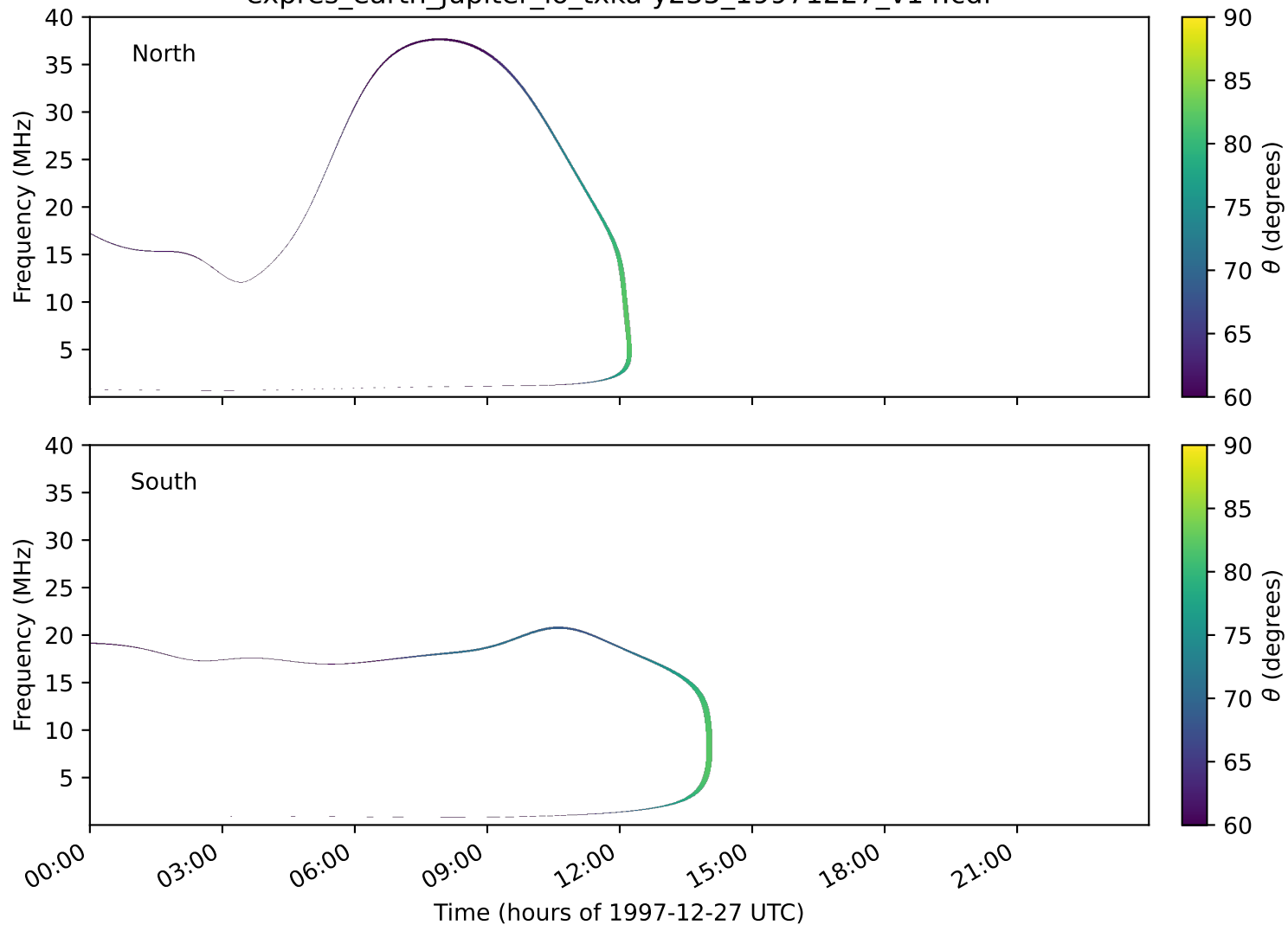
expres_earth_jupiter_io_txka-y235_19971227_v14.cdf
