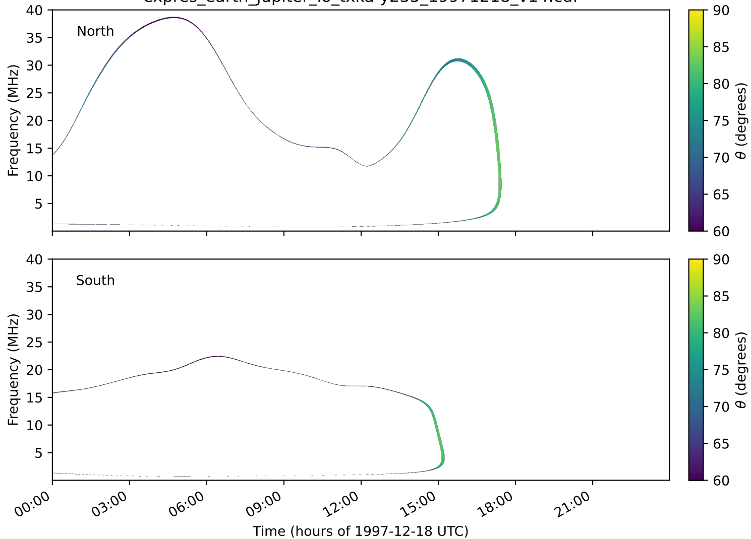
expres_earth_jupiter_io_txka-y235_19971218_v14.cdf
