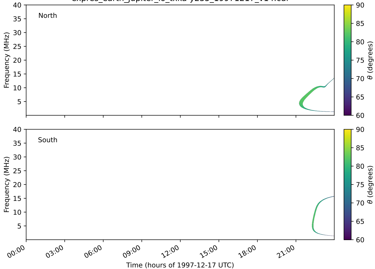
expres_earth_jupiter_io_txka-y235_19971217_v14.cdf
