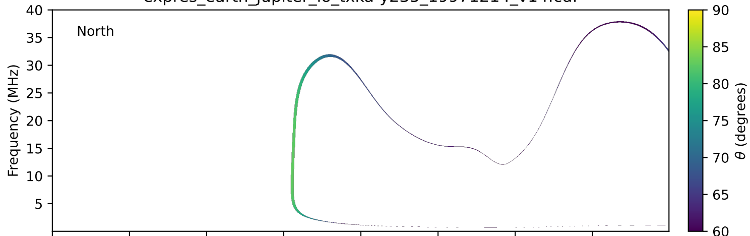
expres_earth_jupiter_io_txka-y235_19971214_v14.cdf
