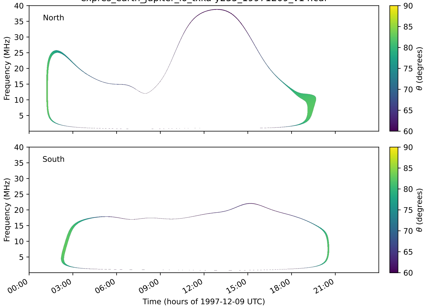
expres_earth_jupiter_io_txka-y235_19971209_v14.cdf
