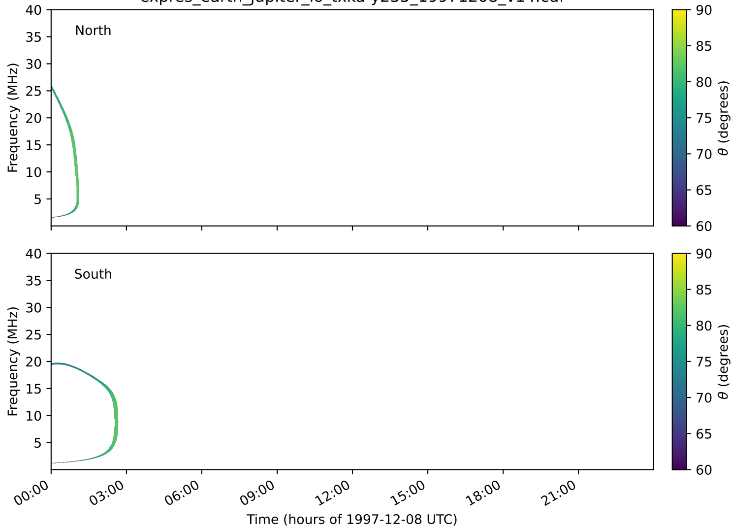
expres_earth_jupiter_io_txka-y235_19971208_v14.cdf
