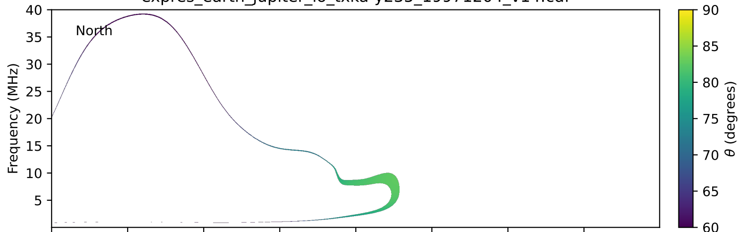
expres_earth_jupiter_io_txka-y235_19971204_v14.cdf
