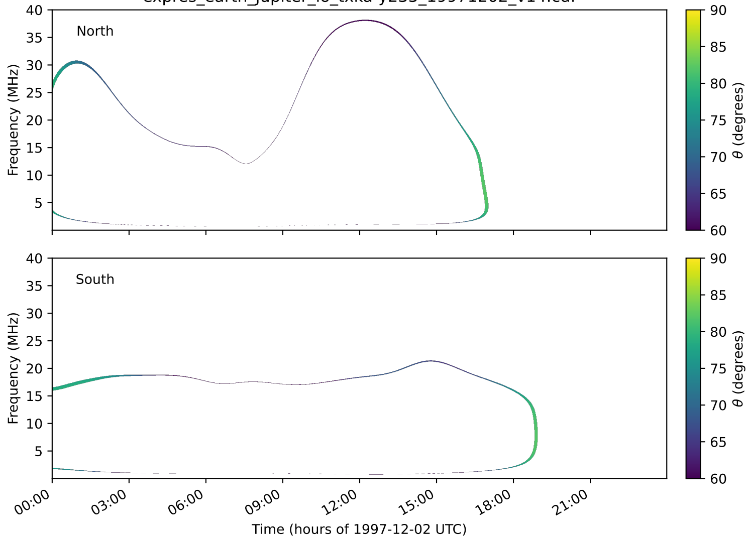
expres_earth_jupiter_io_txka-y235_19971202_v14.cdf
