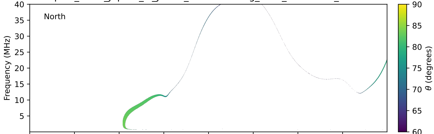
expres_earth_jupiter_io_jrm33_lossc-wid1deg_3kev_19971230_v11.cdf
