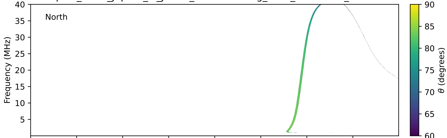
expres_earth_jupiter_io_jrm33_lossc-wid1deg_3kev_19971219_v11.cdf
