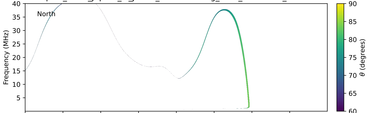
expres_earth_jupiter_io_jrm33_lossc-wid1deg_3kev_19971218_v11.cdf
