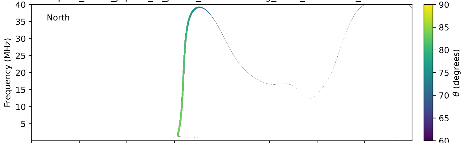
expres_earth_jupiter_io_jrm33_lossc-wid1deg_3kev_19971214_v11.cdf
