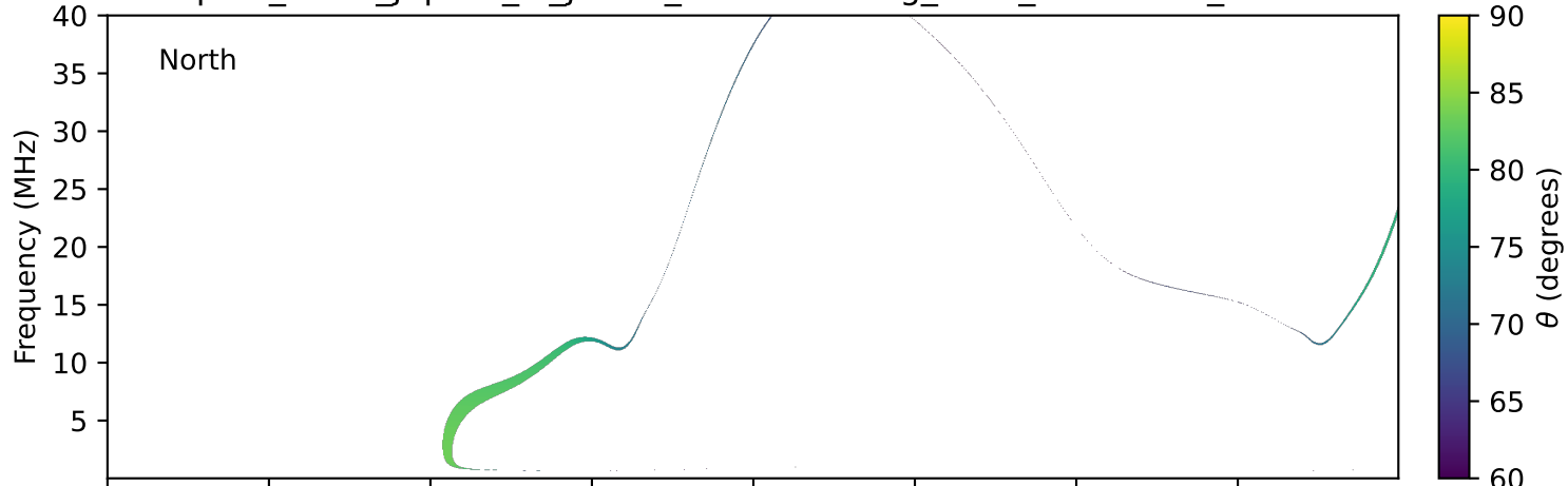
expres_earth_jupiter_io_jrm09_lossc-wid1deg_3kev_19971230_v11.cdf
