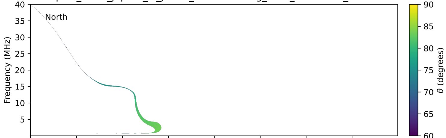
expres_earth_jupiter_io_jrm09_lossc-wid1deg_3kev_19971229_v11.cdf
