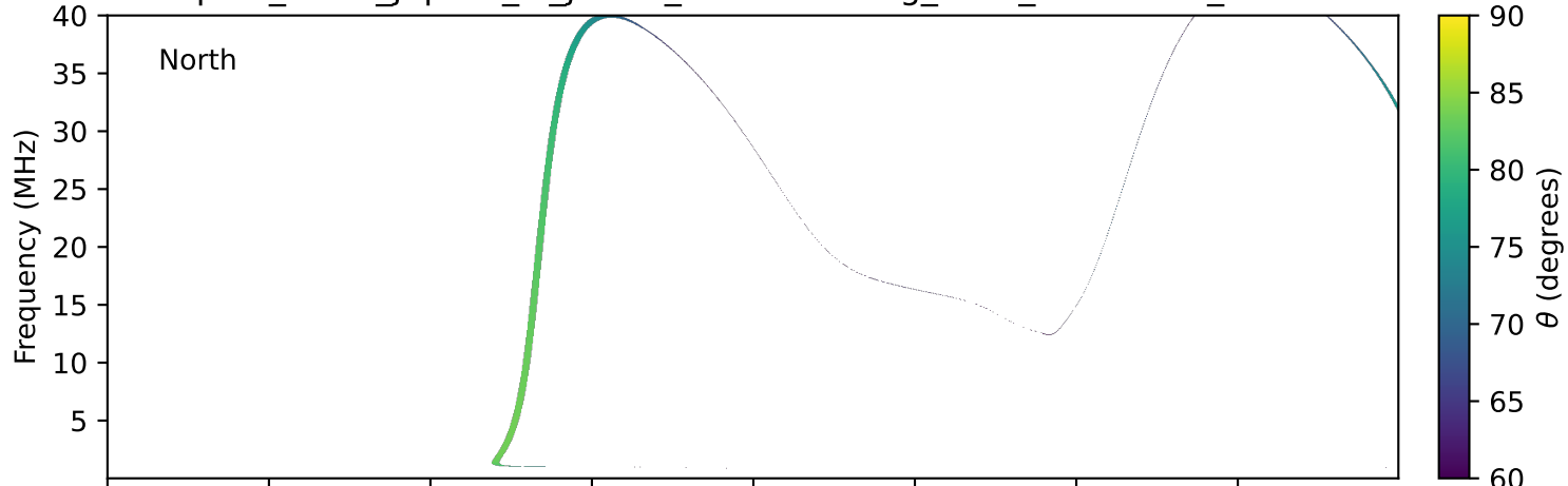
expres_earth_jupiter_io_jrm09_lossc-wid1deg_3kev_19971207_v11.cdf
