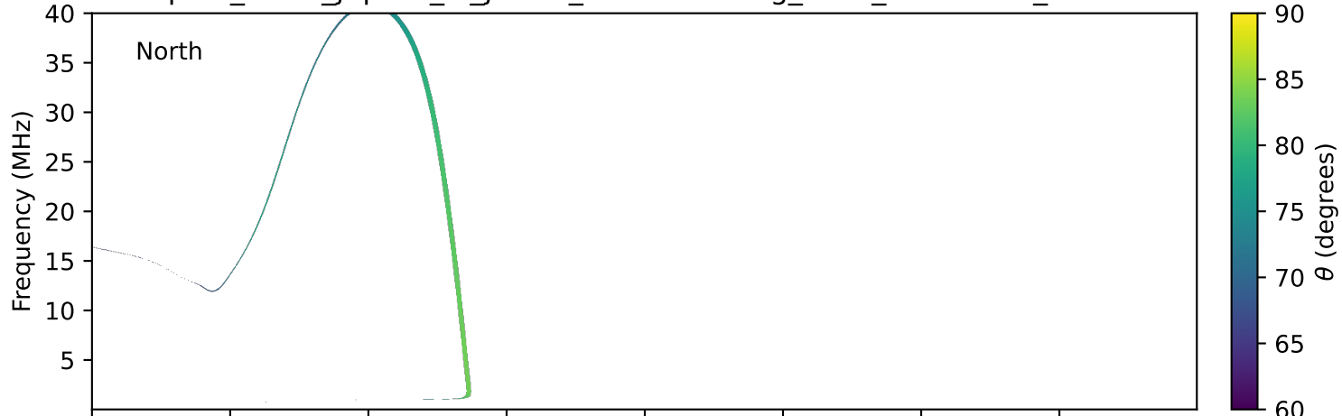
expres_earth_jupiter_io_jrm09_lossc-wid1deg_3kev_19971206_v11.cdf
