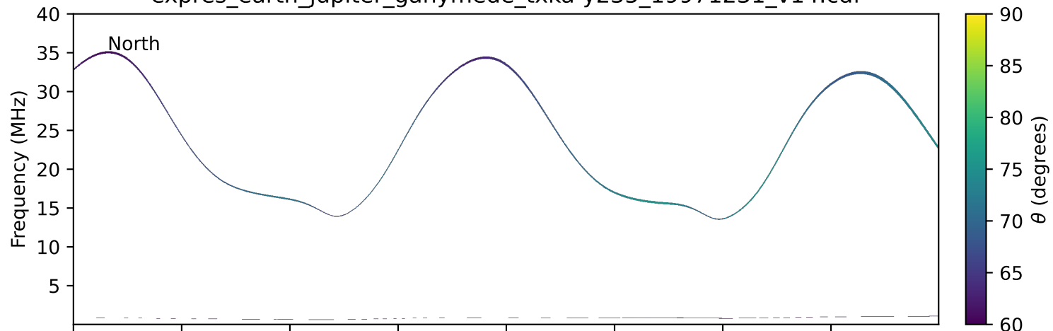
expres_earth_jupiter_ganymede_txka-y235_19971231_v14.cdf
