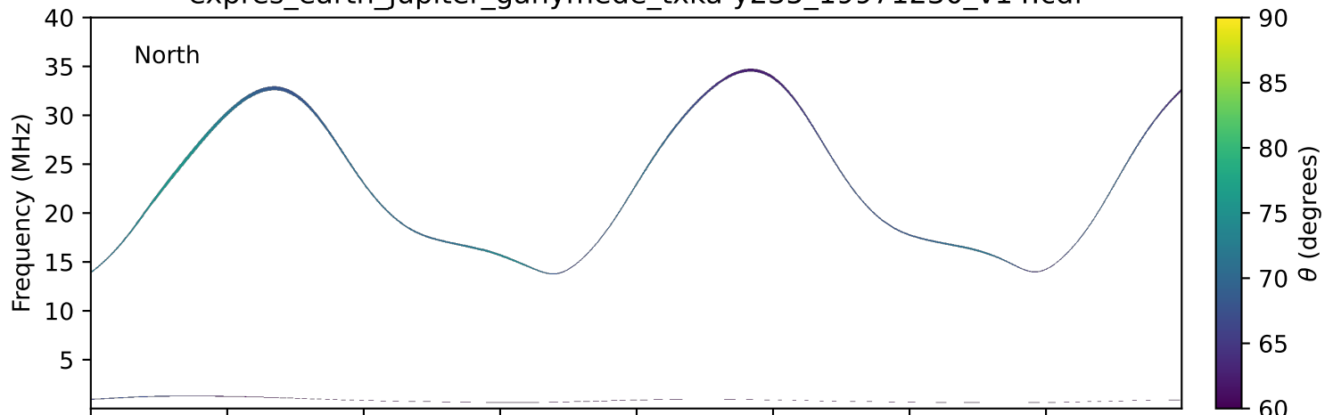
expres_earth_jupiter_ganymede_txka-y235_19971230_v14.cdf
