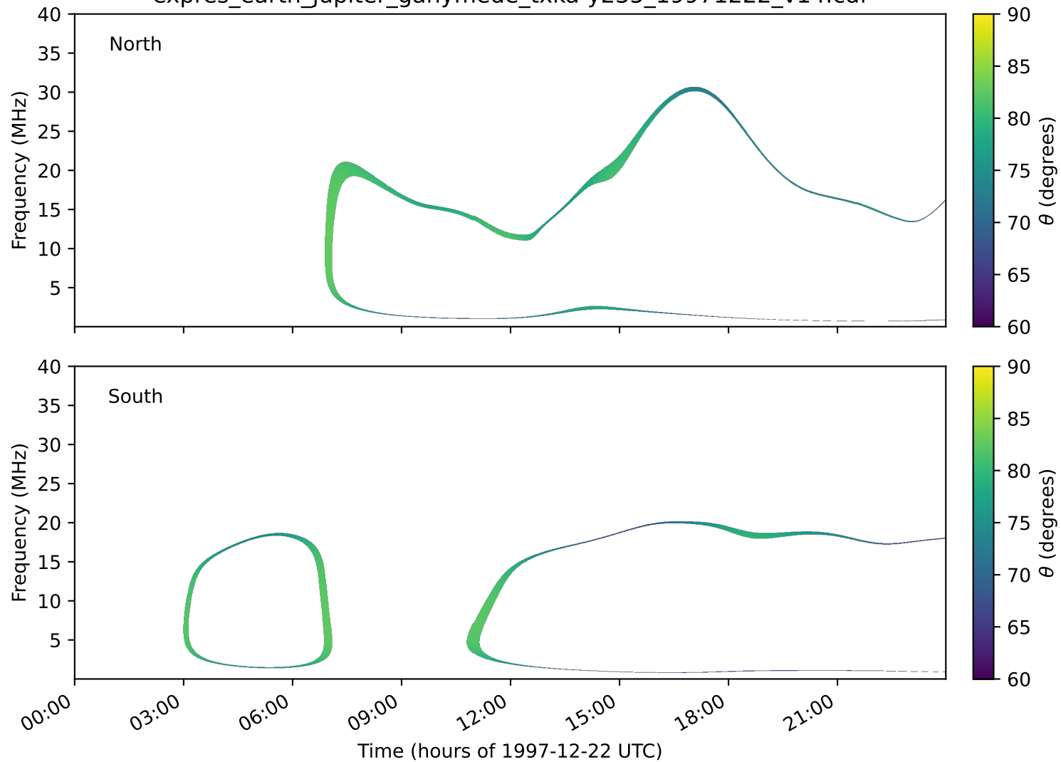
expres_earth_jupiter_ganymede_txka-y235_19971222_v14.cdf
