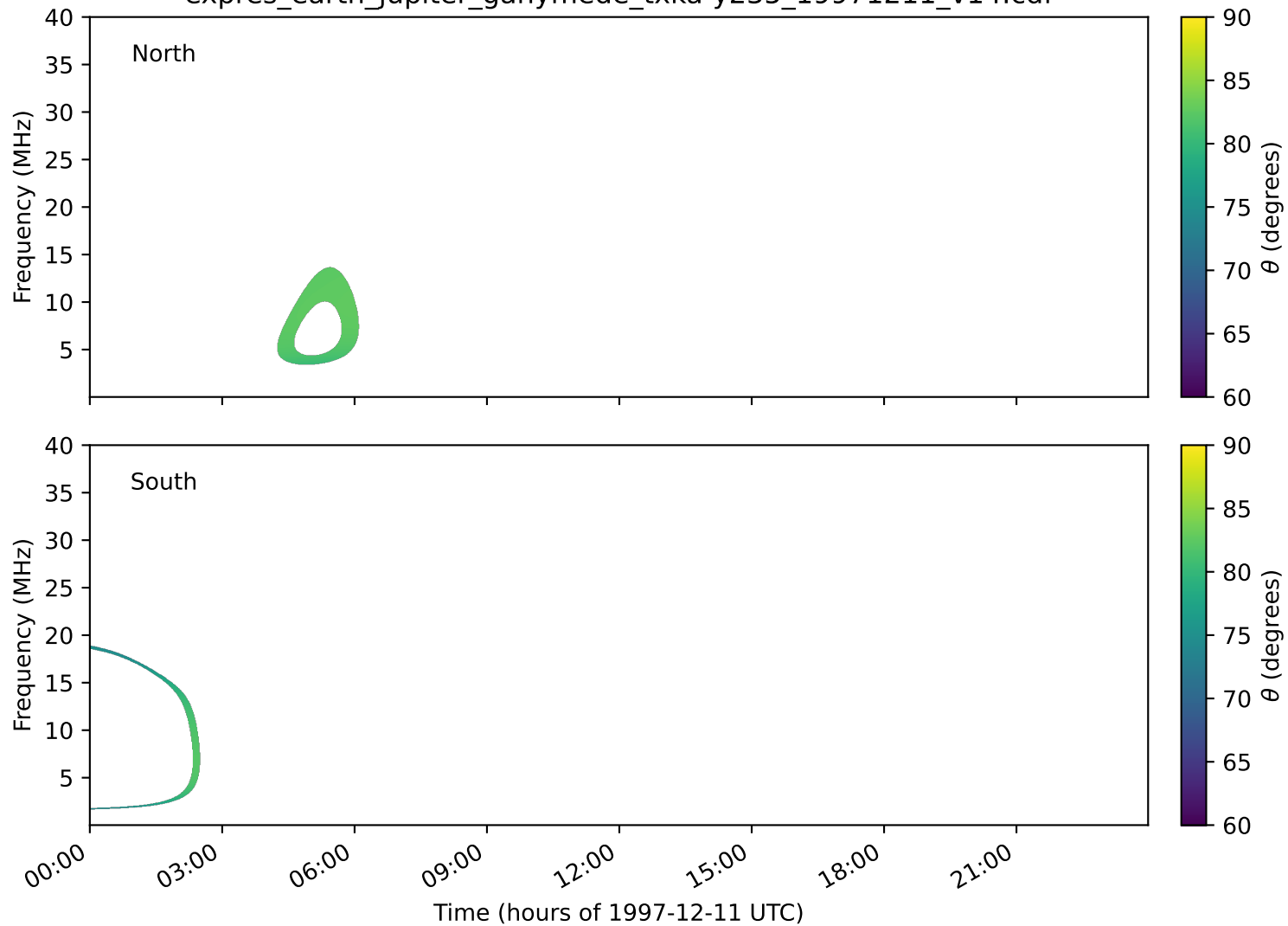
expres_earth_jupiter_ganymede_txka-y235_19971211_v14.cdf
