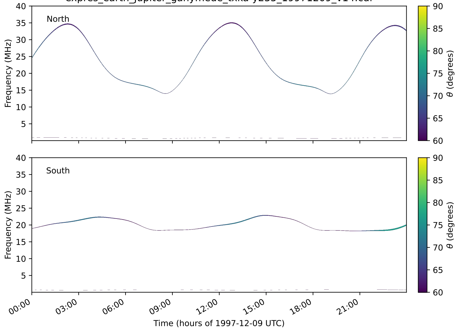
expres_earth_jupiter_ganymede_txka-y235_19971209_v14.cdf
