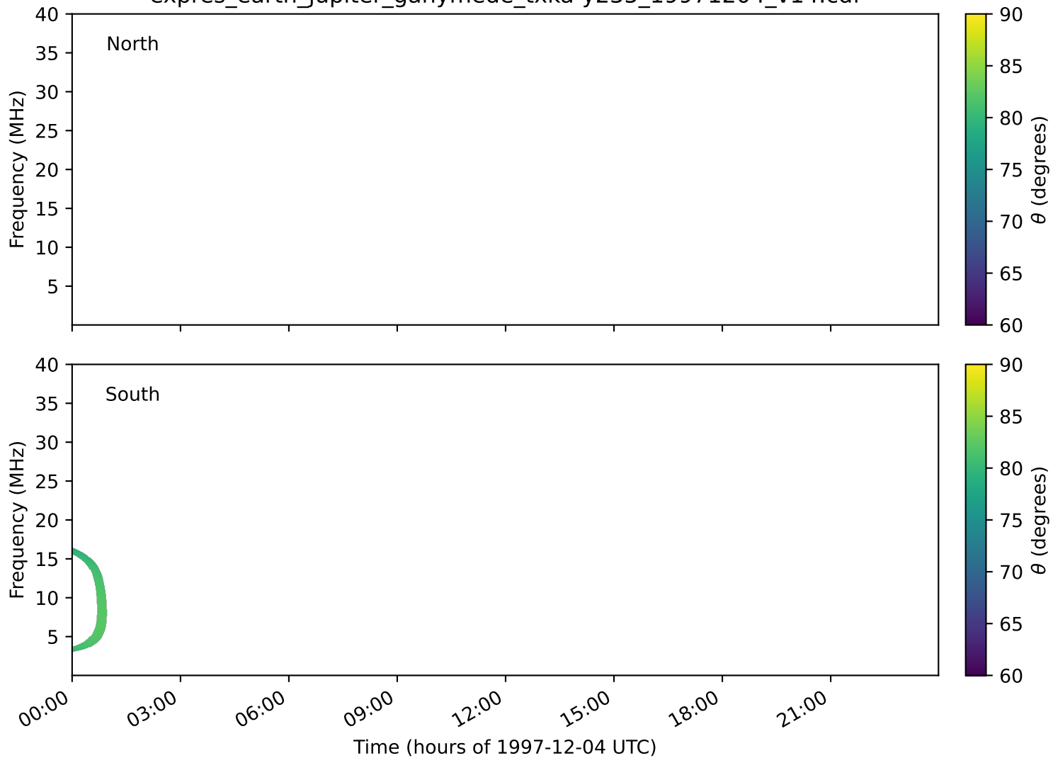
expres_earth_jupiter_ganymede_txka-y235_19971204_v14.cdf
