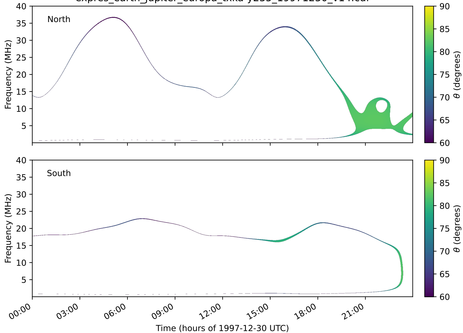
expres_earth_jupiter_europa_txka-y235_19971230_v14.cdf
